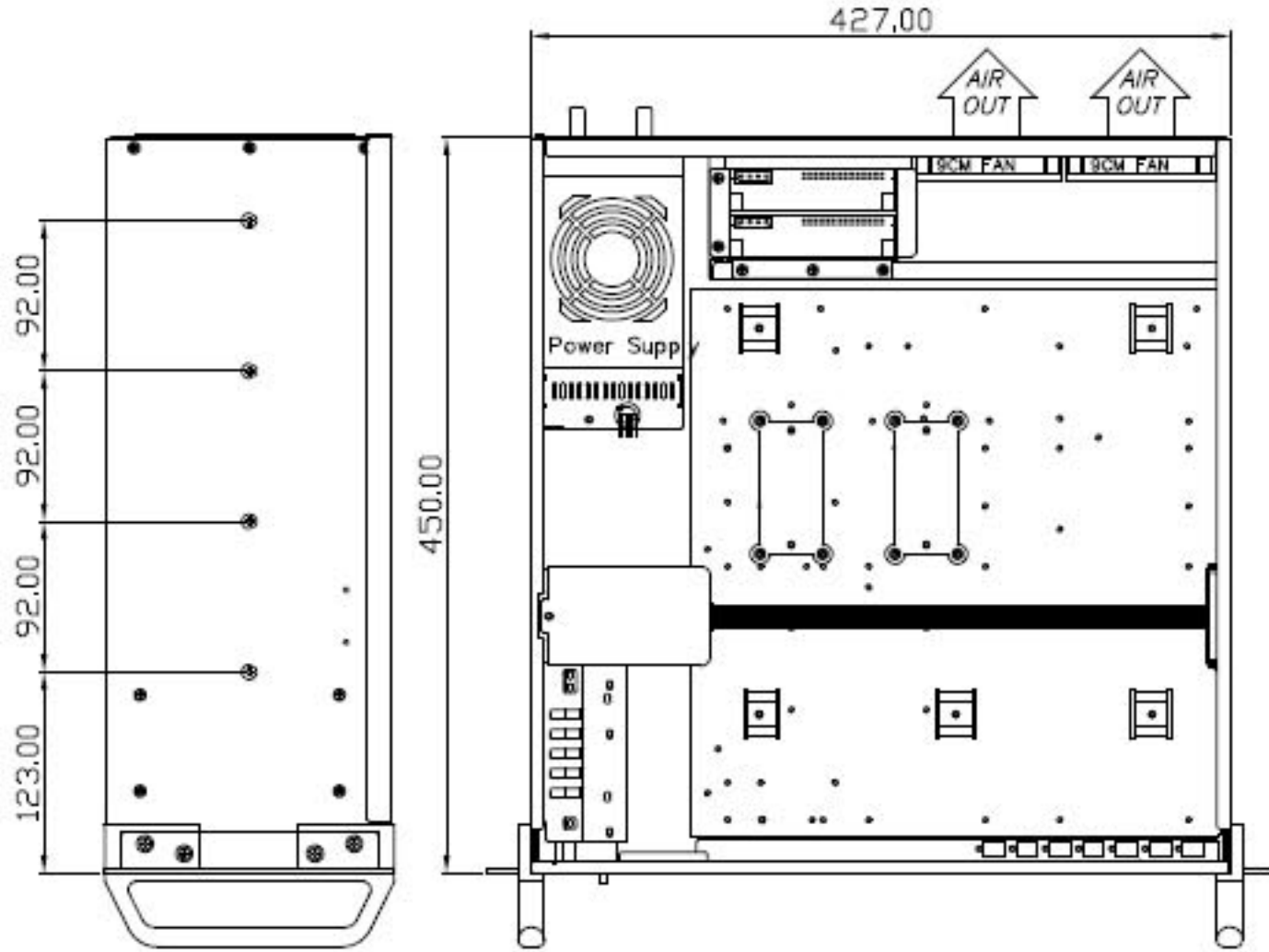
Left-side View
