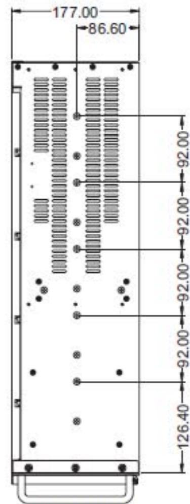
Right-side View
