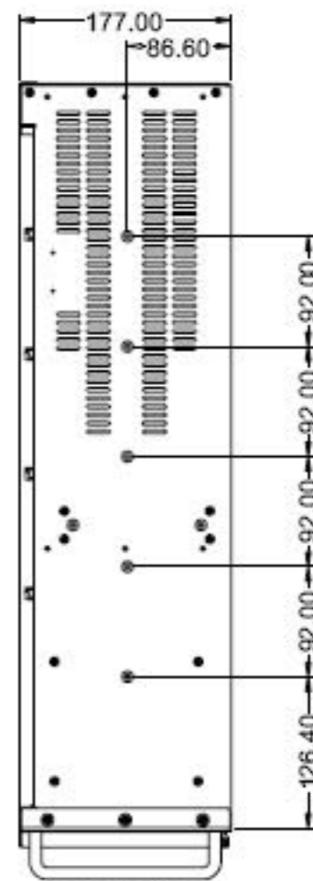
Right-side View
