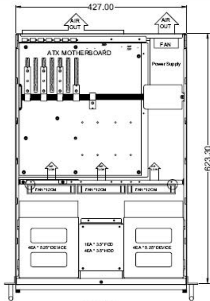
Top View
