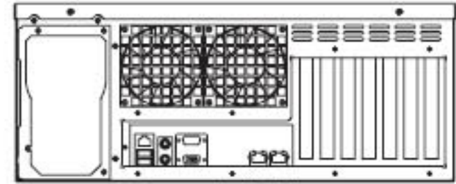
Rear out-side View
