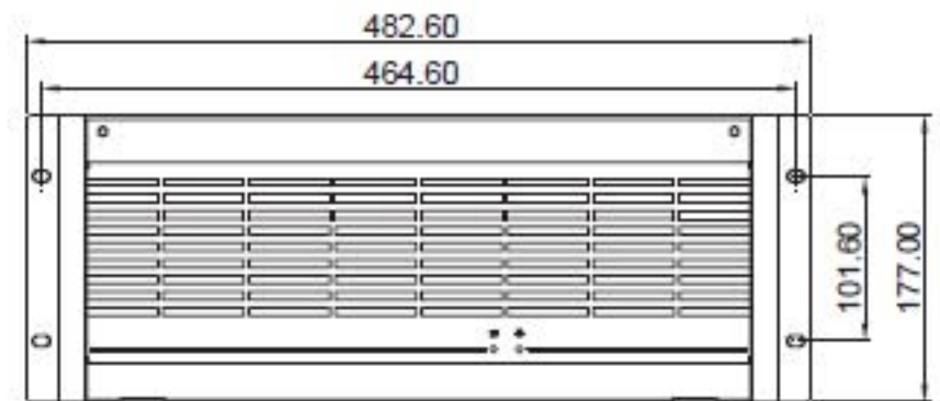
Front out-side View
