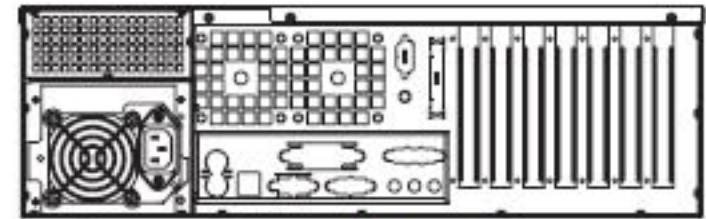
Rear View
