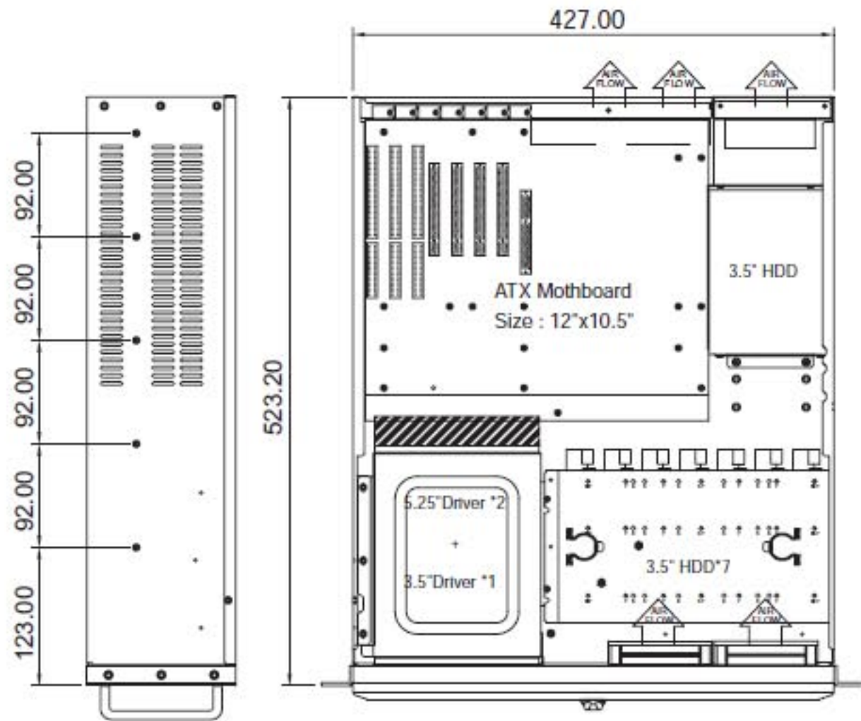
Left-side View
