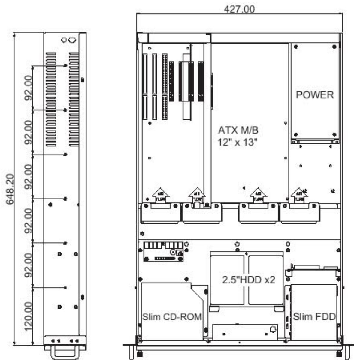
Left-side View
