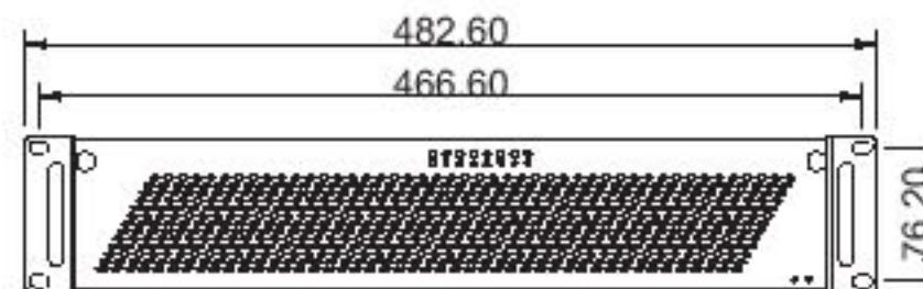
Front out-side View
