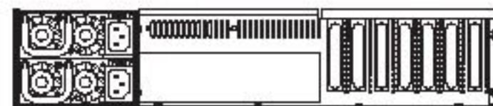
Rear View (GHI-280V)
