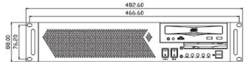
Front View
