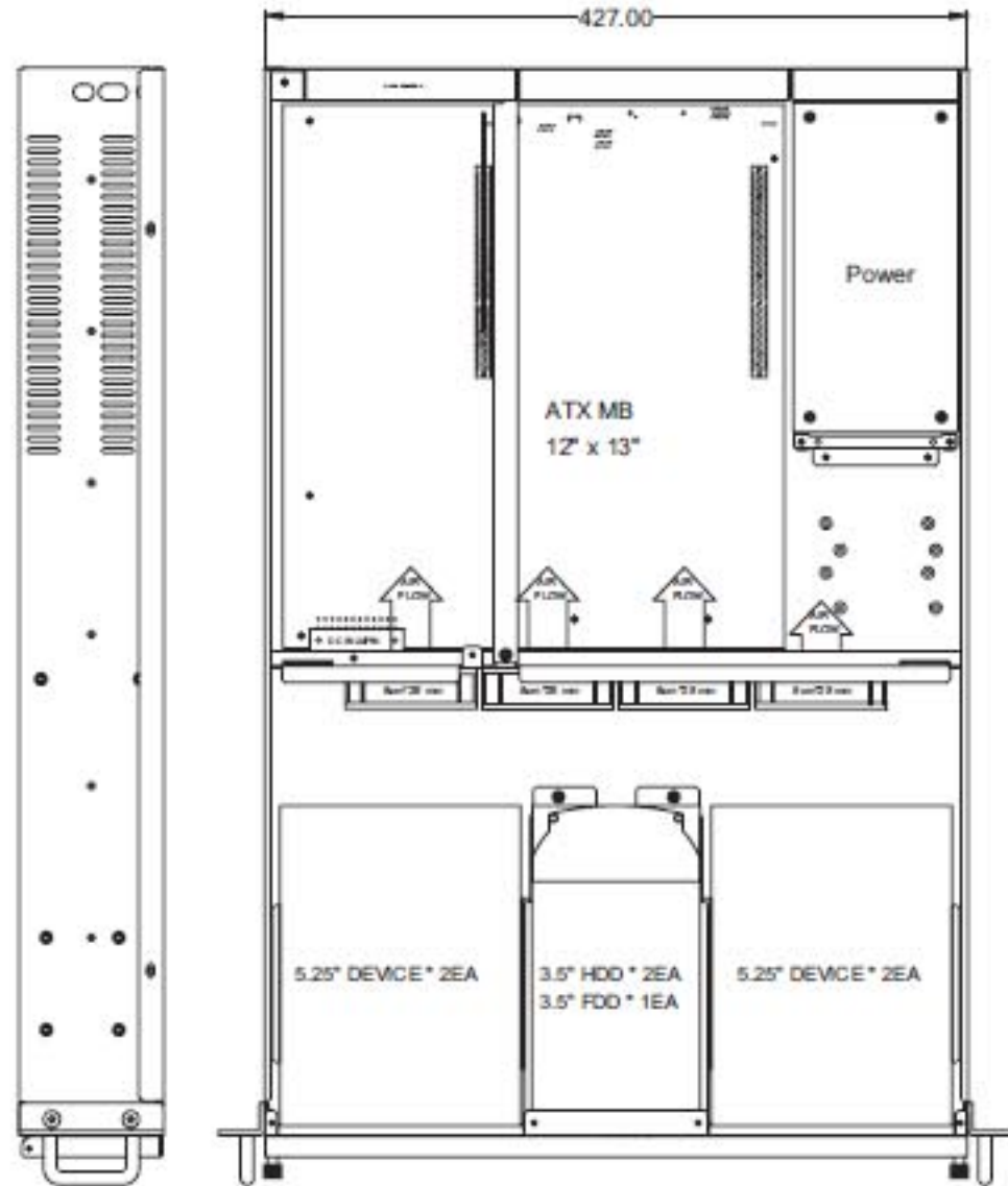
Left-side View
