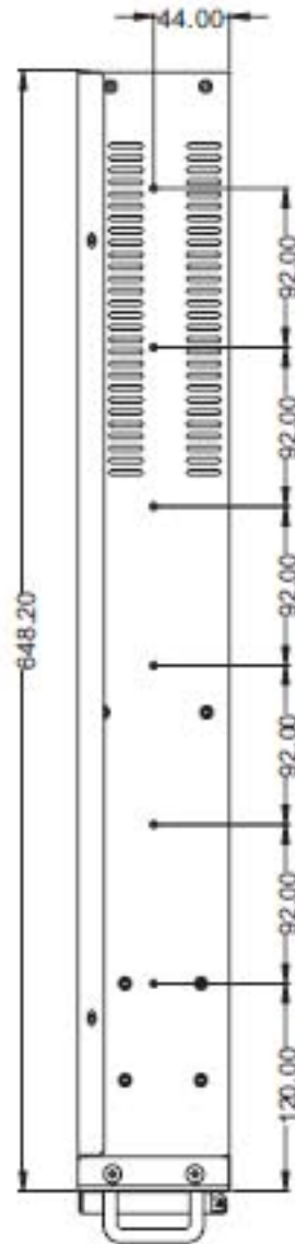
Right-side View
