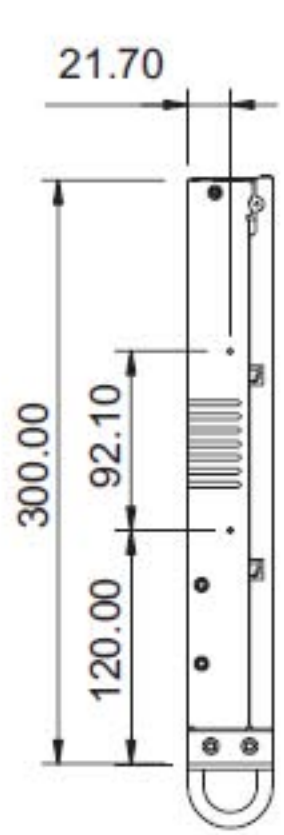
Left-side View
