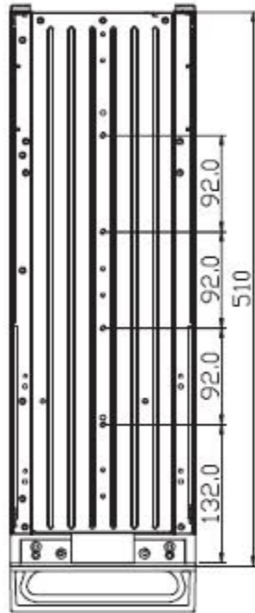
Left View
