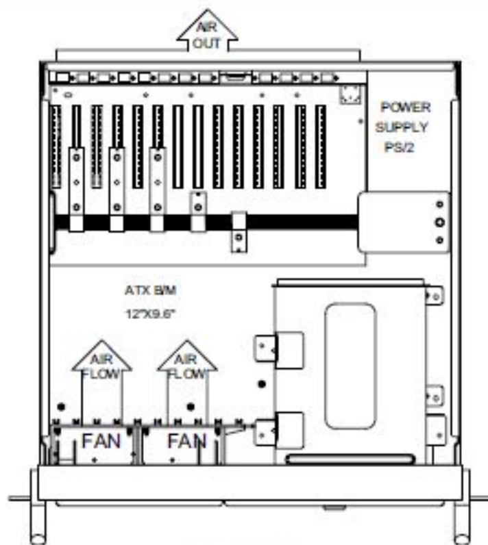
Top View
