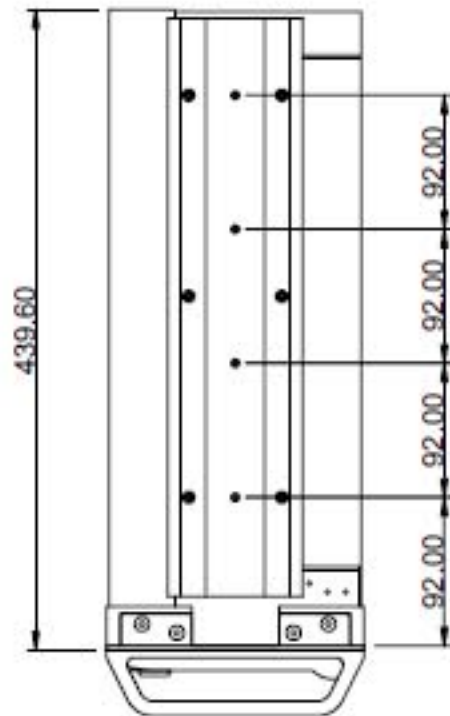
Right-side View
